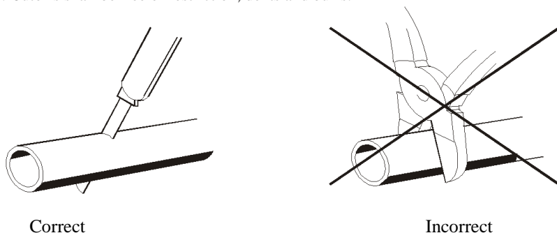
Figure 11 – Cutting the fuel pipe before installation
