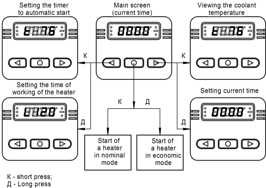
Figure 6.3 - Algorithm of operation of the control panel.
