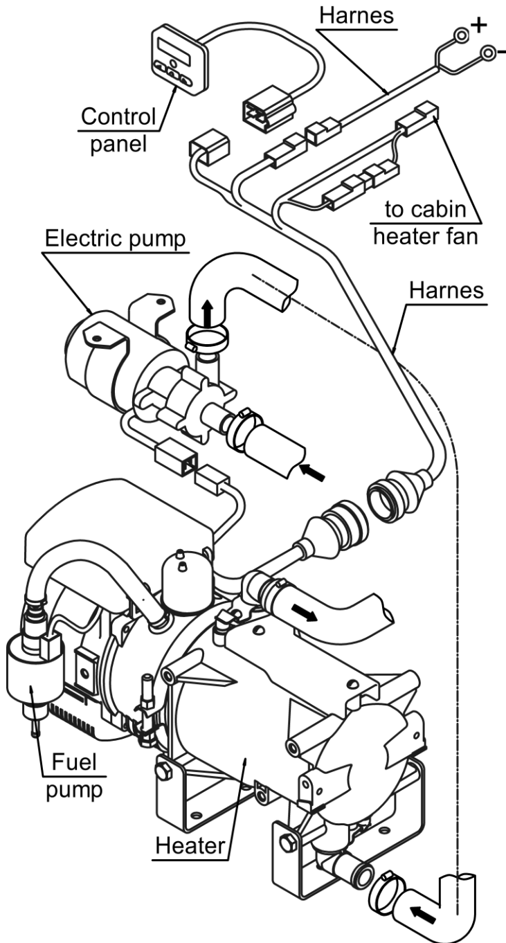
Figure 4.2 – Pre-heater main components
