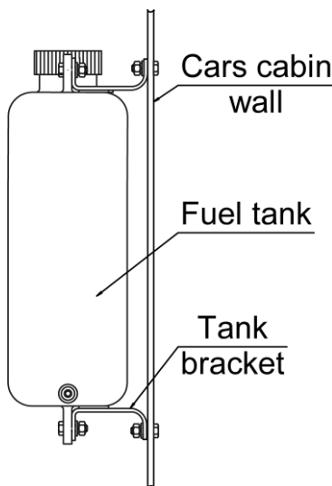
Figure 8-Fuel tank installation on vehicle
