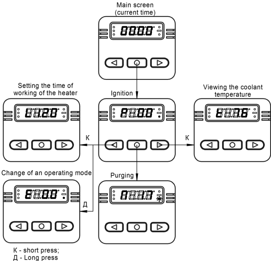
Figure 6.7 Start of a heater in nominal mode.
