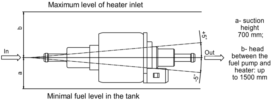
Figure 10 – Allowable installation position of the fuel pump
