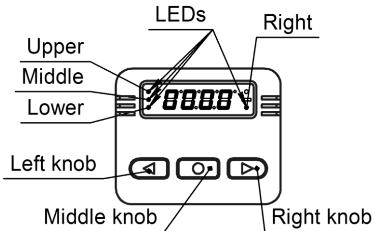
Figure 6.2-Control panel
