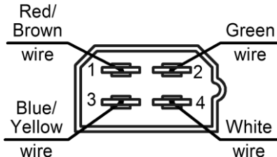
Figure. 6.1 – Installation contacts in the connector
